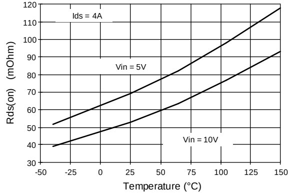
Fig. 4 - On Resistance vs. Temperature
