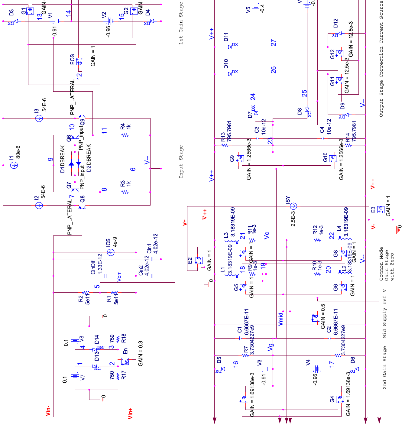
FIGURE 64. SPICE SCHEMATIC
