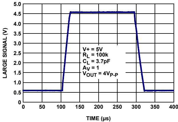
FIGURE 52. CHARACTERIZED LARGE SIGNAL STEP RESPONSE (4V)
