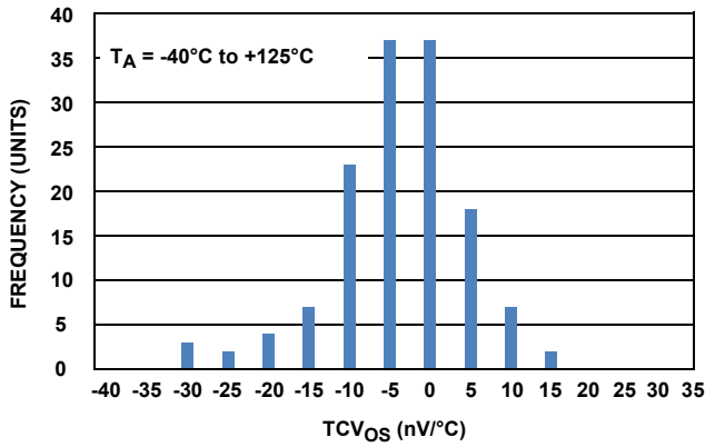
FIGURE 36. TCV_{OS} HISTOGRAM
