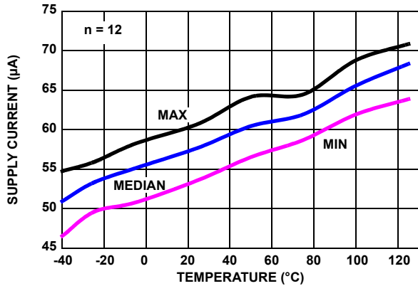
FIGURE 23. ISL28176 SUPPLY CURRENT vs TEMPERATURE V_S = \pm 2.5V ENABLED, R_L = INF
