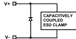
CIRCUIT 4
