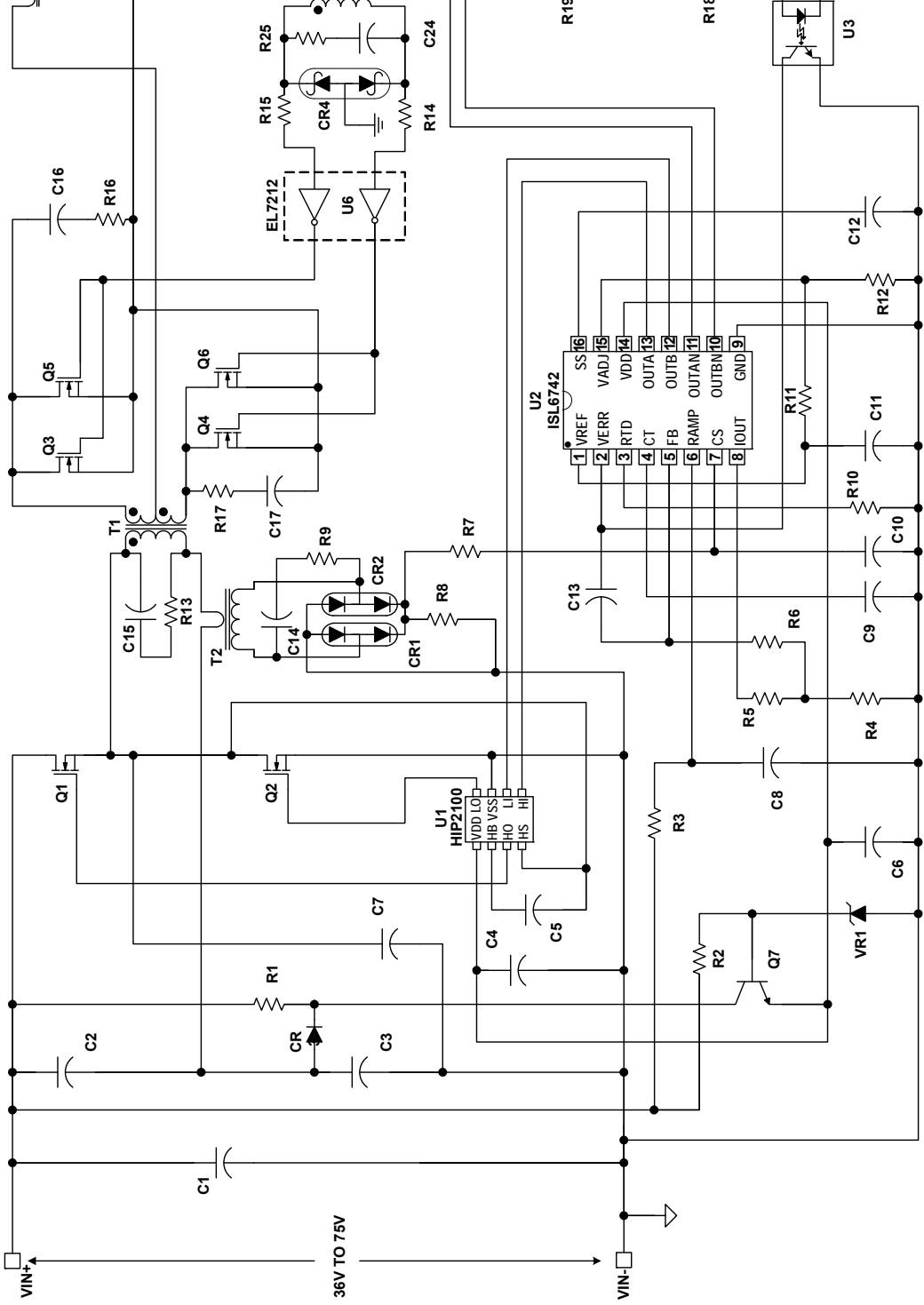
FIGURE 2. TELECOM PRIMARY SIDE CONTROL HALF-BRIDGE CONVERTER WITH SYNCHRONOUS RECTIFICATION
