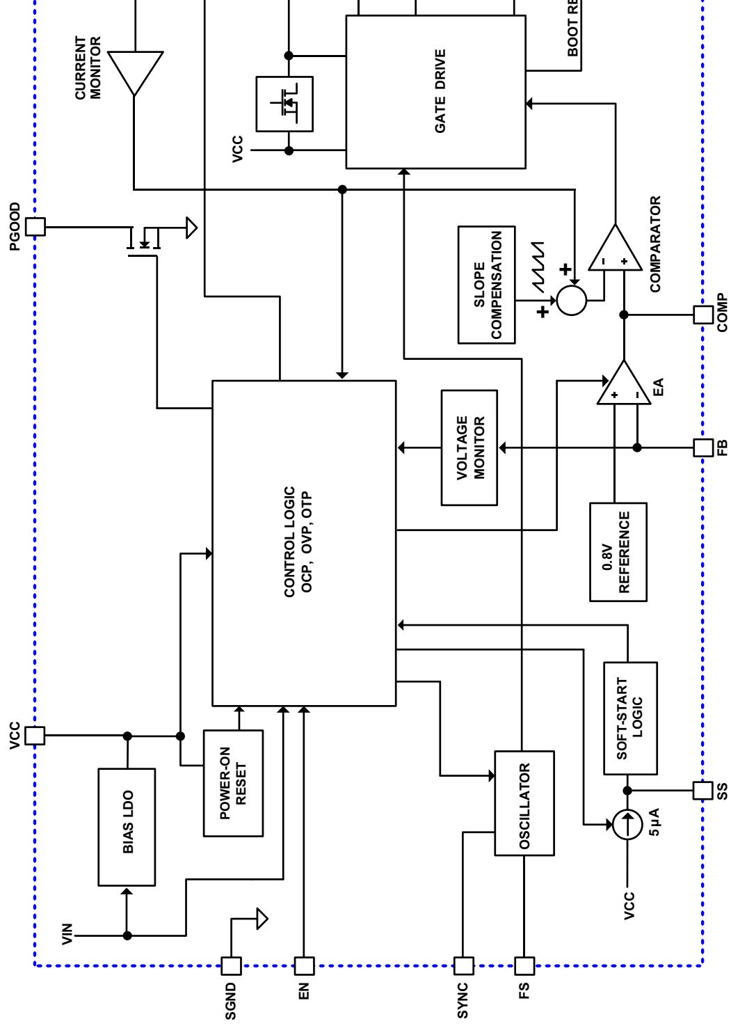
FIGURE 3. BLOCK DIAGRAM
