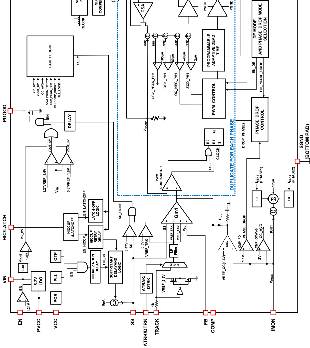
FIGURE 3. BLOCK DIAGRAM
