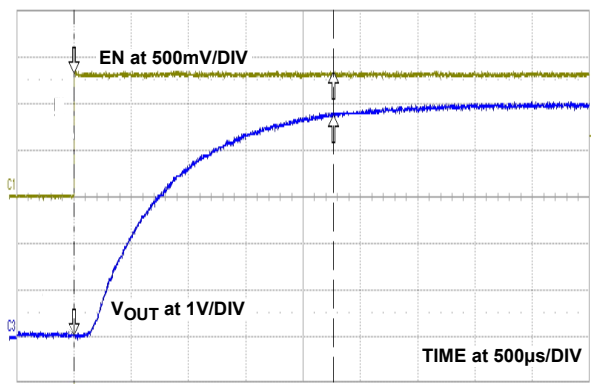
FIGURE 9. START-UP WAVEFORM
