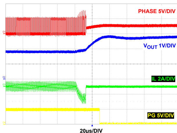
FIGURE 46. OVERVOLTAGE PROTECTION
