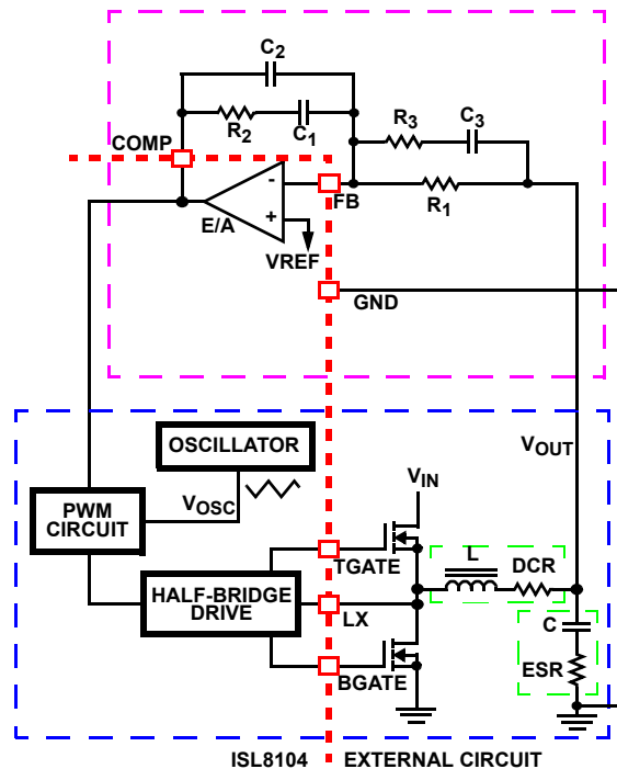
FIGURE 7. VOLTAGE-MODE BUCK CONVERTER COMPENSATION DESIGN
