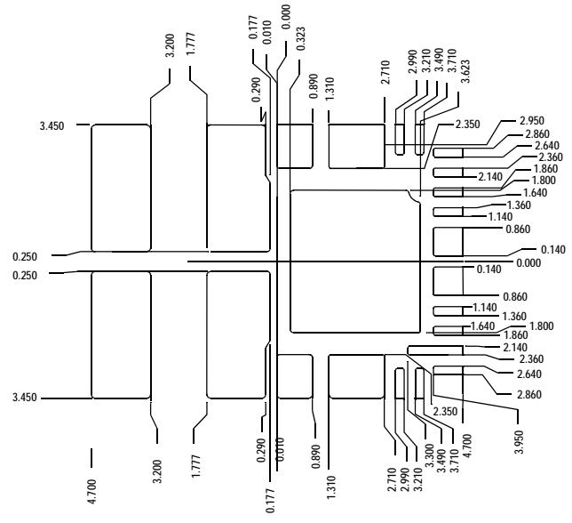
STENCIL PATTERN WITH 23 MOSLP TOP VIEW
