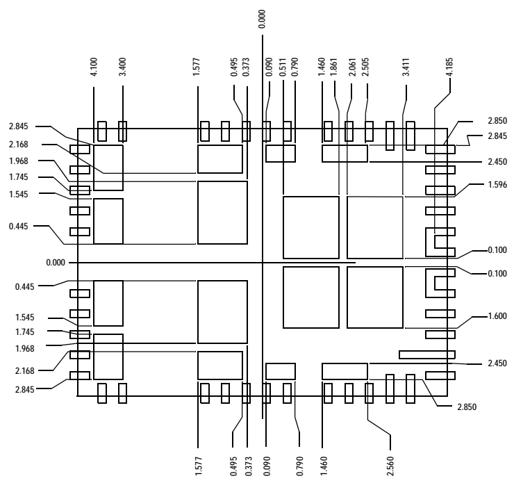
STENCIL PATTERN WITH 23 MOSLP TOP VIEW
