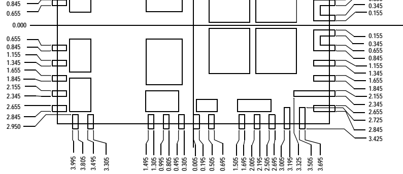
STENCIL PATTERN WITH 23
