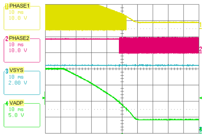
FIGURE 9. ADAPTER VOLTAGE RAMP DOWN, BUCK -> BUCK-BOOST -> BOOST OPERATION MODE TRANSITION
