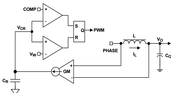
Figure 24. R3 Modulator
