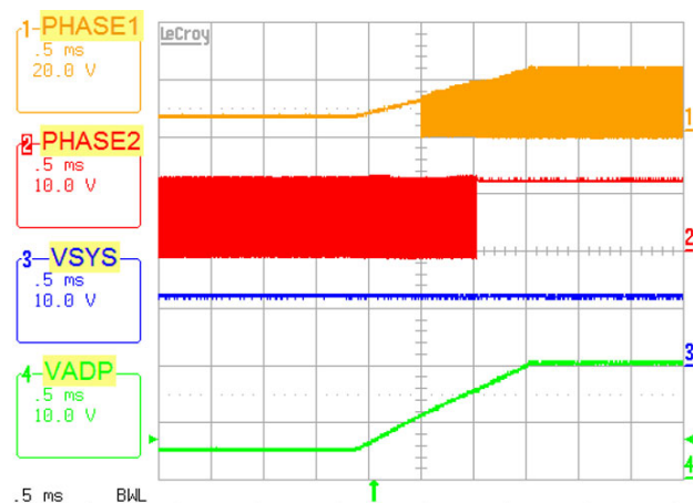
Figure 8. ADP Voltage Ramps Up in Reverse Mode, Buck -> Buck-Boost -> Boost Operation Mode Transition
