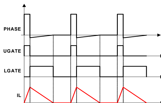
Figure 27. Diode Emulation
