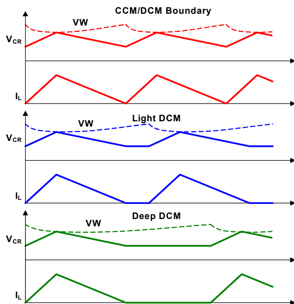
Figure 28. Period Stretching
