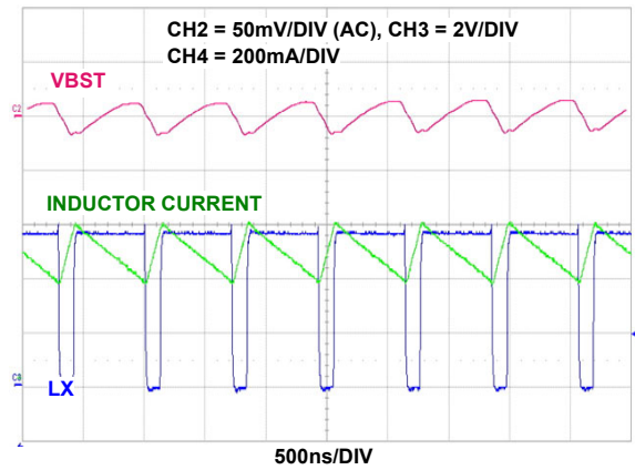
FIGURE 13. VBST RIPPLE, 150mA LOAD, VBST = 5.65V
