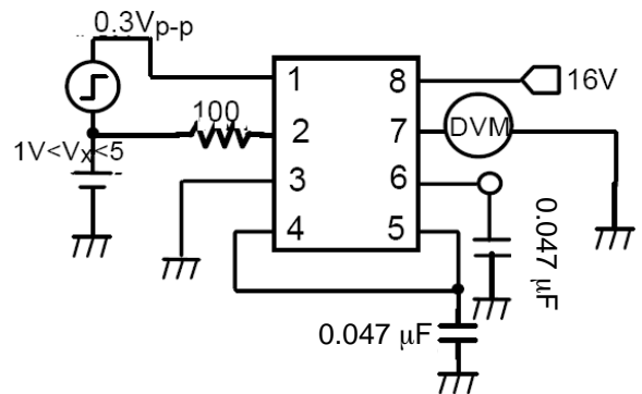
Figure 18. Response Time
