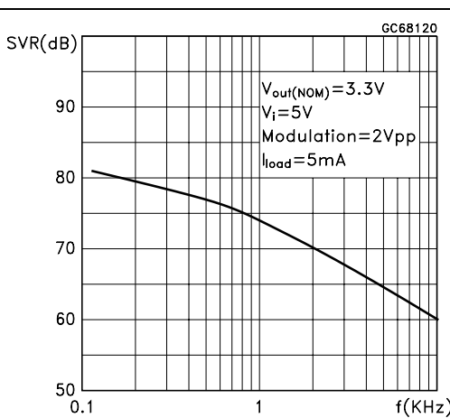
Figure 9. SVR vs frequency
