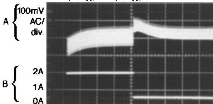
Figure 23. Horizontal Time Base: 200 μs/div.
