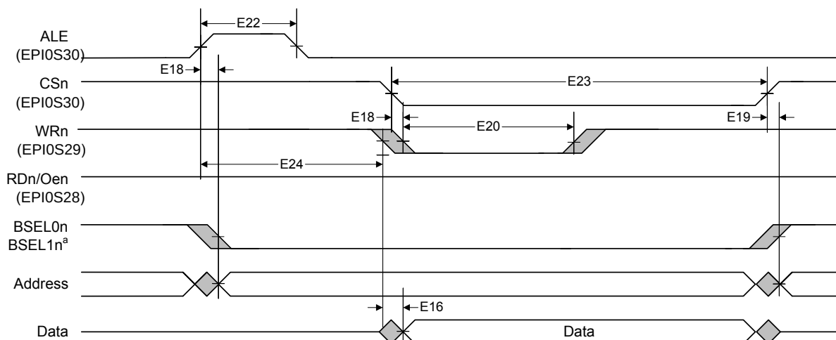
Figure 25-21. Host-Bus 8/16 Mode Write Timing
