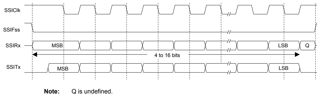
Figure 15-7. Freescale SPI Frame Format (Single Transfer) with SPO=1 and SPH=0
