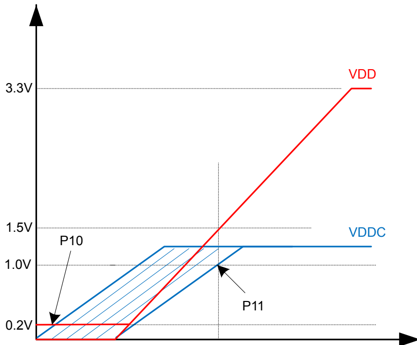
Figure 25-7. Voltage Requirements When Using an External V DDC Source
