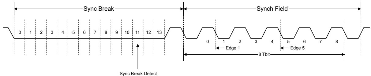
Figure 14-5. LIN Synchronization Field
