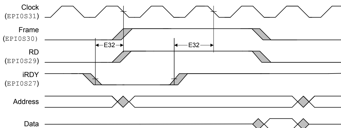
Figure 25-25. General-Purpose Mode iRDY Timing
