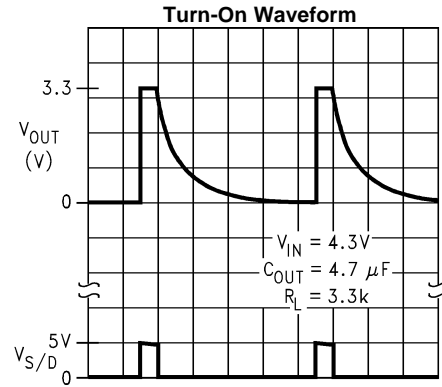
20 ms/Div Figure 18.
