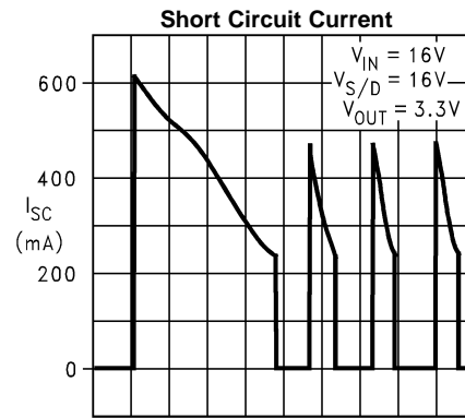
200 ms/Div Figure 20.
