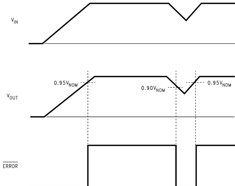
Figure 22. \overline{\text{Error}} Flag Operation
