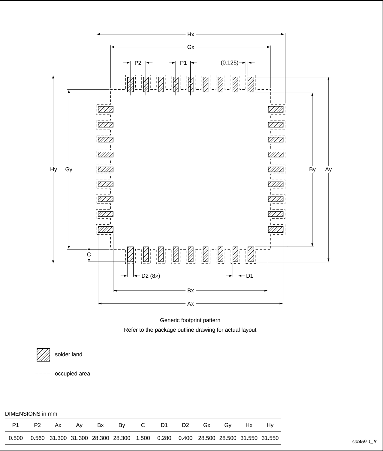
Fig 56. Reflow soldering of the LQFP208 package
