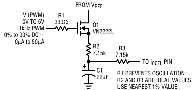
LT1183 I CCFL PWM Programming with V REF
