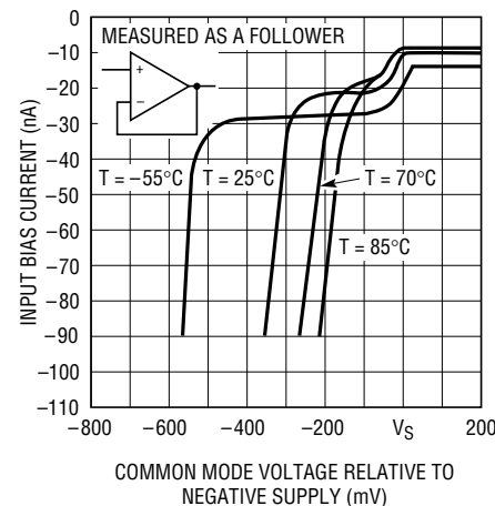
LT1218/19 • F03
