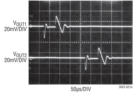
Channel-to-Channel Isolation
