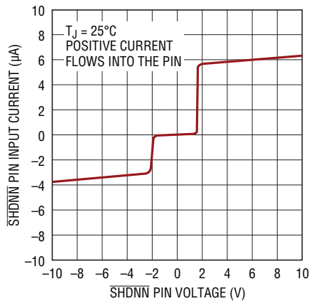
\overline{SHDNN} Pin Input Current
