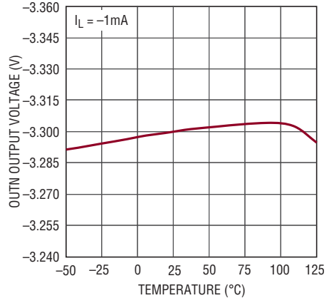
LT3032-3.3 OUTN Output Voltage
