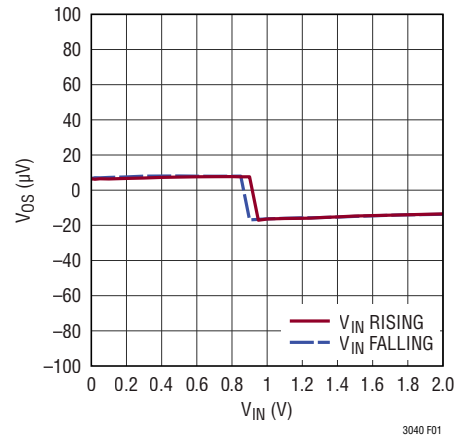
Figure 1. PNP to NPN Diff Pair Transition
