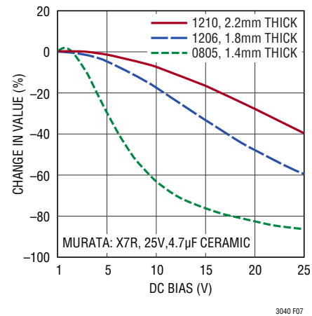
Figure 7. Capacitor Voltage Coefficient for Different Case Sizes
