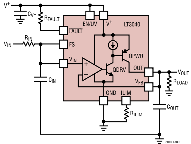
Figure 9. Low Pass Filter with Fast-Startup Disabled
