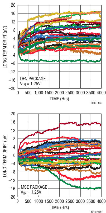
Figure 13. LT3040 Long Term Drift
