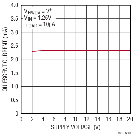
Quiescent Current
