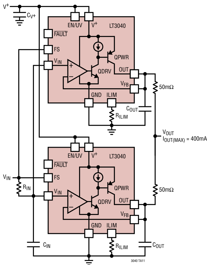
Figure 11. Parallel Devices
