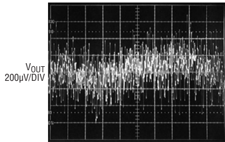
C_{OUT} = 10\mu\text{F} I_{LOAD} = 500\text{mA} V_{OUT} = 5\text{V}
