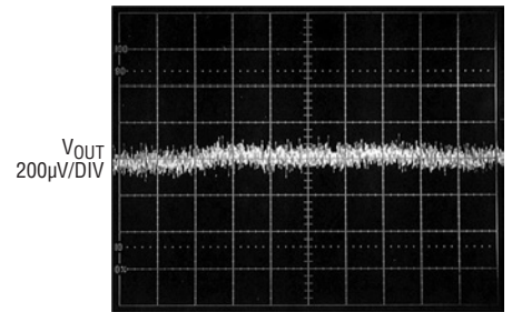
C_{OUT} = 10\mu\text{F} I_{LOAD} = 500\text{mA} V_{OUT} = 5\text{V}
