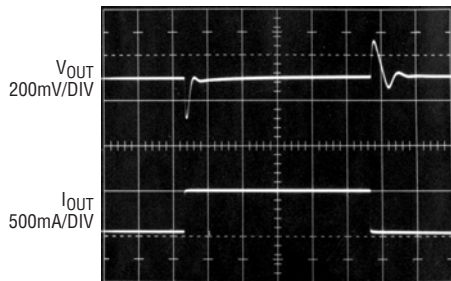
V_{IN} = 6\text{V} C_{OUT} = 10\mu\text{F} I_{FB-DIVIDER} = 10\mu\text{A} V_{OUT} = 5\text{V}
