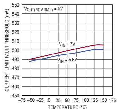
Precision Current Limit, R_{I_{MAX}} = 604\Omega
