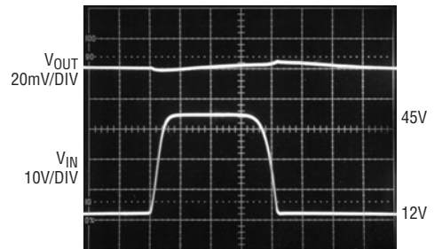
V_{OUT} = 5\text{V} I_{OUT} = 100\text{mA} C_{OUT} = 10\mu\text{F}
