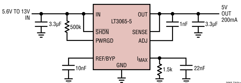
5V Supply with 200mA Precision Current Limit
