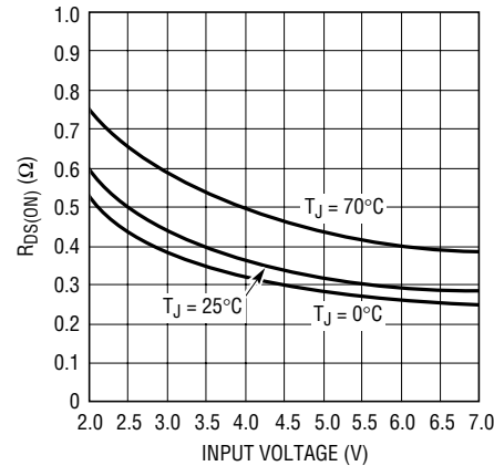
Switch Resistance
