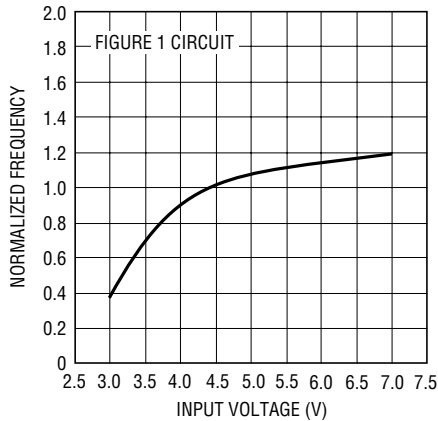
Operating Frequency
