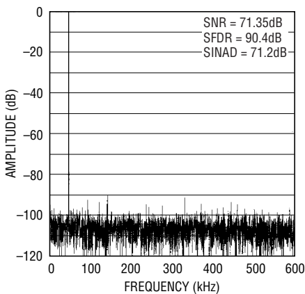
Nonaveraged 4096 Point FFT, f_{IN} = 47\text{kHz} , Bipolar Mode, PGA = 0, LTC1851
