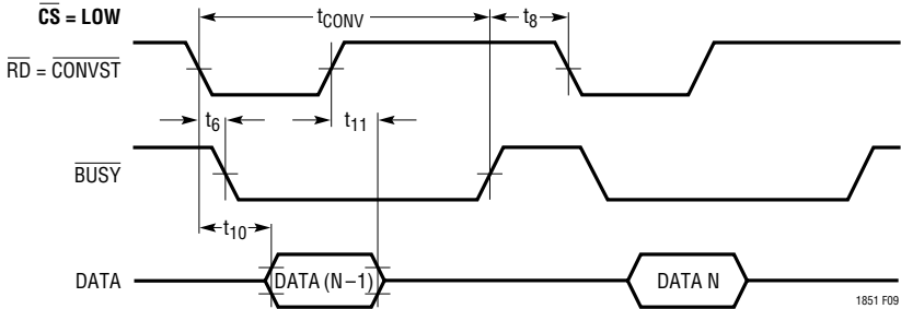
Figure 9. ROM Mode Timing
