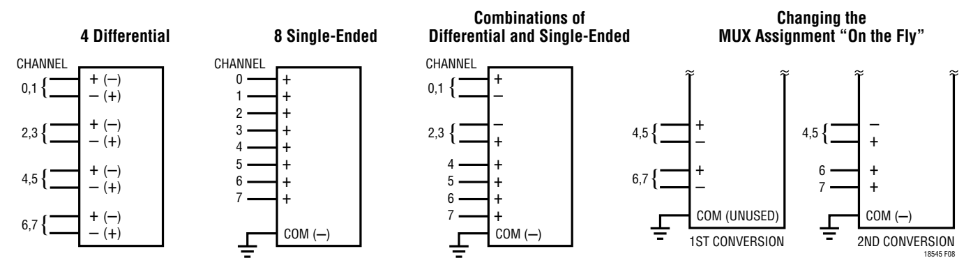
Figure 8. Examples of Multiplexer Options on the LTC1854/LTC1855/LTC1856
