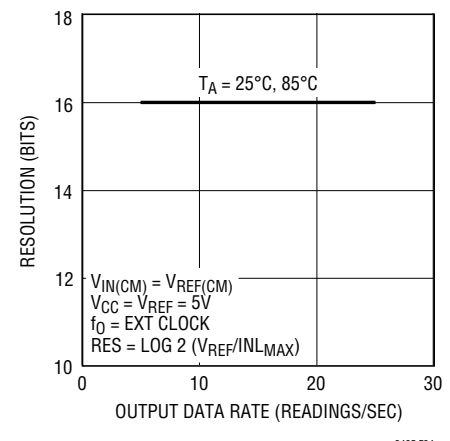
Figure 34. Resolution ( INL_{MAX} \le 1LSB ) vs Output Data Rate and Temperature
