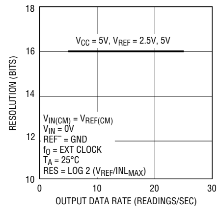
Figure 37. Resolution ( INL_{MAX} \le 1LSB ) vs Output Data Rate and Reference Voltage
