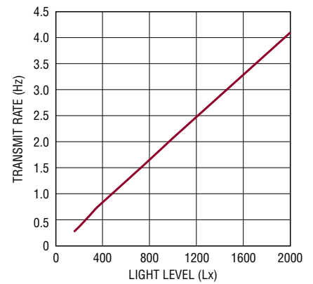
Transmit Rate vs Light Level (Fluorescent)
