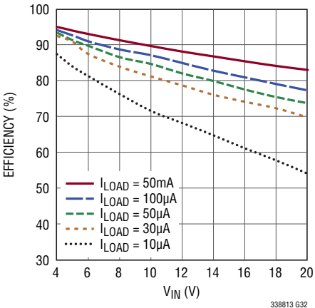
Efficiency vs V_{IN} for V_{OUT} = 3.3\text{V} , L = 22\mu\text{H} (LTC3388-3)
