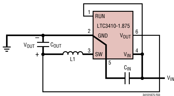
BOLD LINES INDICATE HIGH CURRENT PATHS
