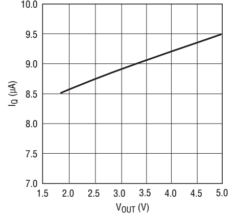
Burst Mode Quiescent Current vs V OUT
