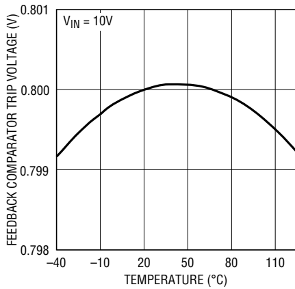
Feedback Comparator Trip Voltage vs Temperature
