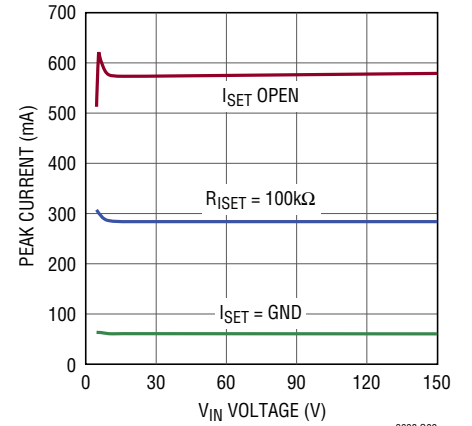
Peak Current Trip Threshold vs Input Voltage
