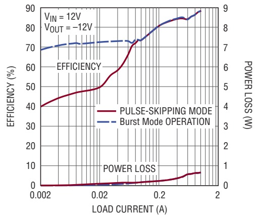
-12V Efficiency
