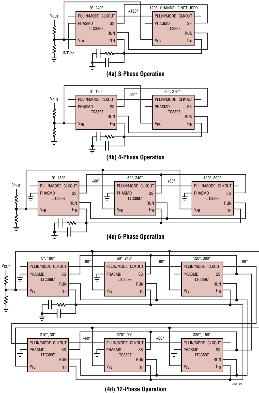
Figure 4. PolyPhase Operation
