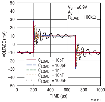
Small-Signal Response
