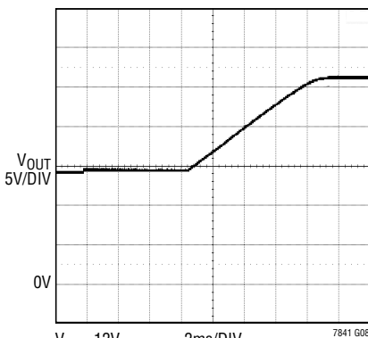
Soft Start-Up
