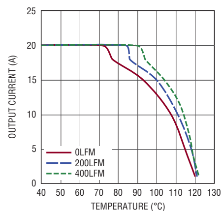
Figure 17. 5V IN to 2.5V OUT with Heat Sink
