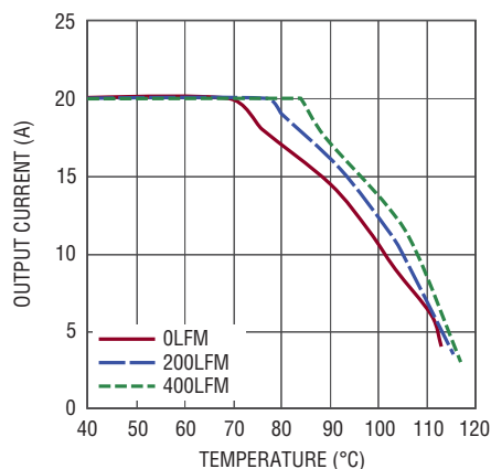
Figure 16. 12V IN to 2.5V OUT No Heat Sink
