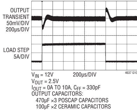
2.5V Transient Response
