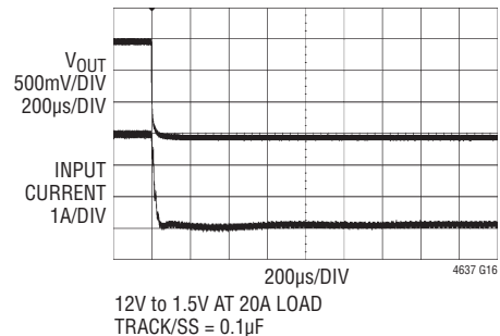
Short-Circuit Protection with 20A Load
