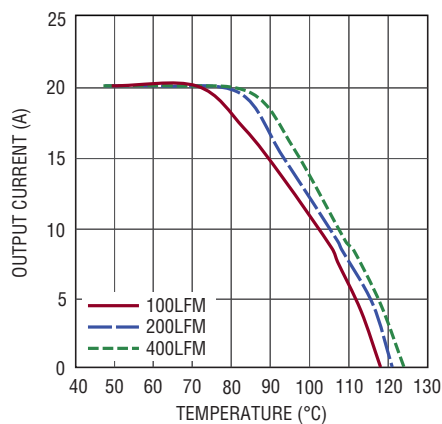
Figure 13. 5V IN to 1.0V OUT with Heat Sink
