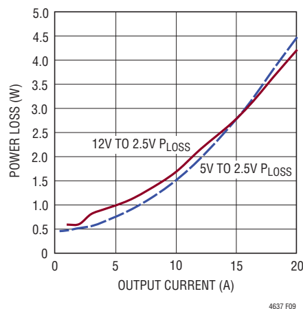
Figure 9. 2.5V OUT Power Loss
