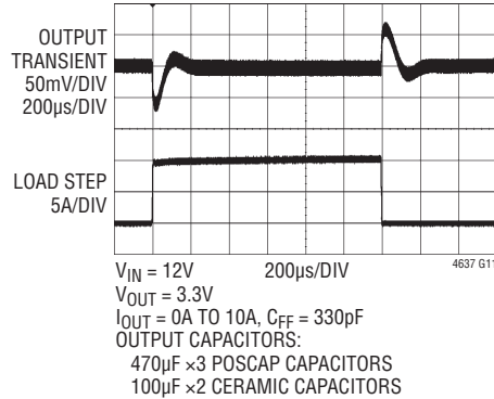
3.3V Transient Response
