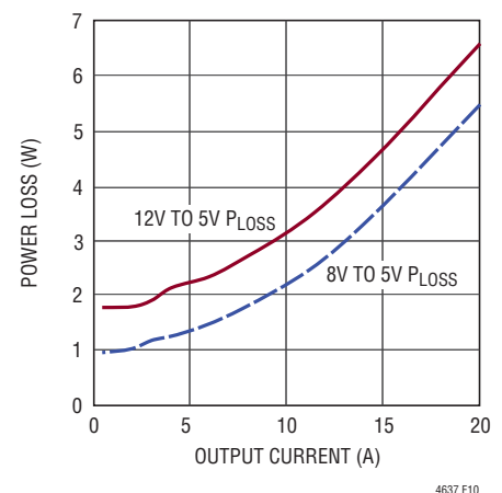
Figure 10. 5V OUT Power Loss
