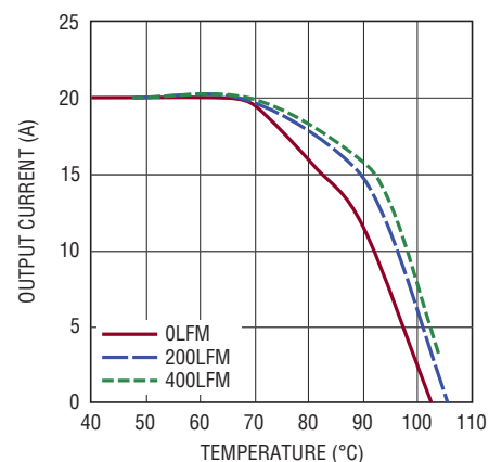
Figure 12. 12V IN to 1.0V OUT No Heat Sink
