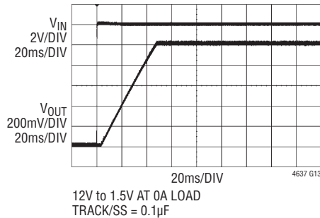
Turn-On No Load
