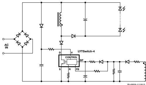
Figure 3d. Typical Buck-Boost Schematic.
