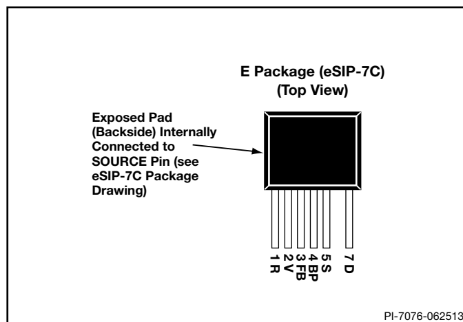
Figure 5. Pin Configuration.
