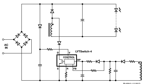
Figure 3b. Typical Buck Schematic.
