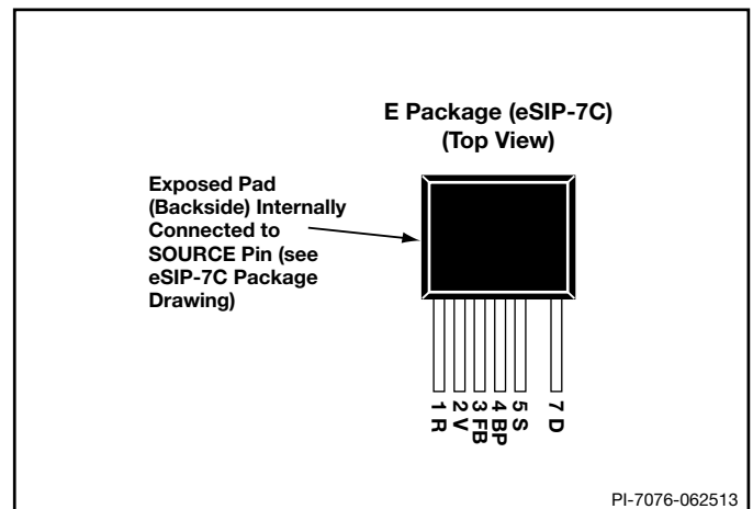
Figure 5. Pin Configuration.
