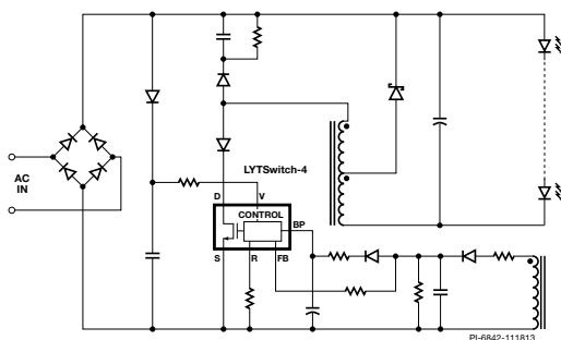
Figure 3c. Typical Tapped Buck Schematic.
