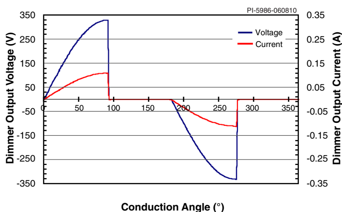
Figure 12. Ideal Dimmer Output Voltage and Current Waveforms for a Trailing Edge Dimmer at 90° Conduction Angle.
