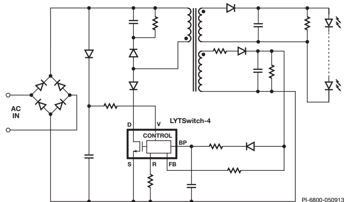
Figure 1. Typical Schematic.
