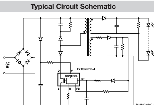
Figure 3a. Typical Isolated Flyback Schematic.
