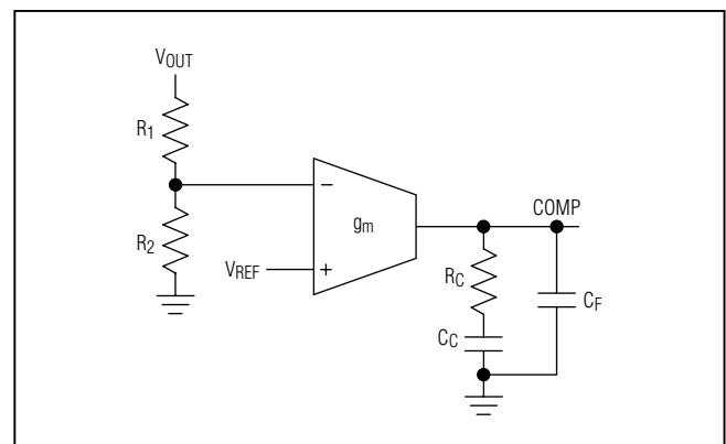
Figure 3. Compensation Network
