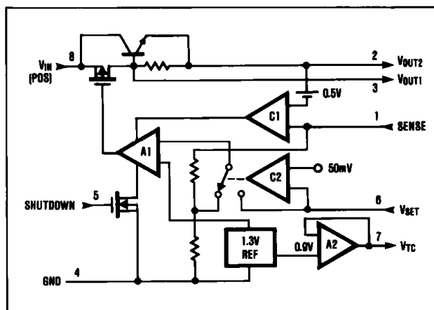
Figure 1. MAX663 Positive Regulator, Block Diagram
