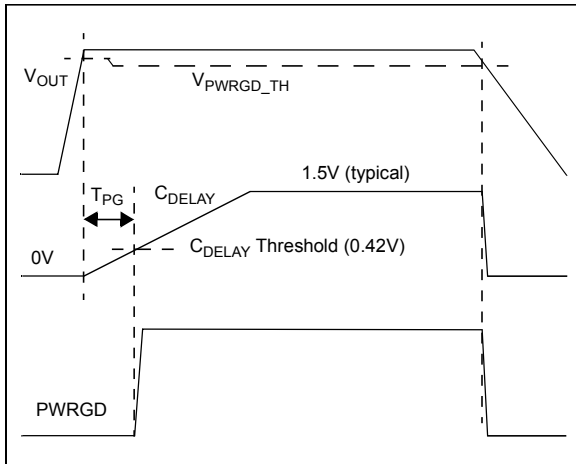
FIGURE 4-4: C_{\text{DELAY}} and PWRGD Timing Diagram.
