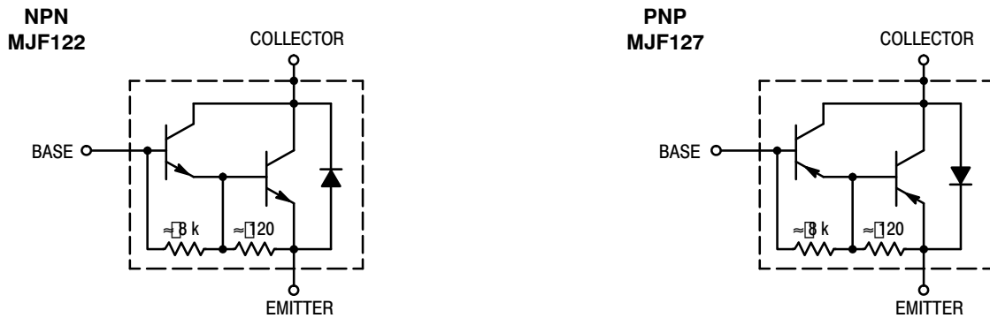
Figure 13. Darlington Schematic
