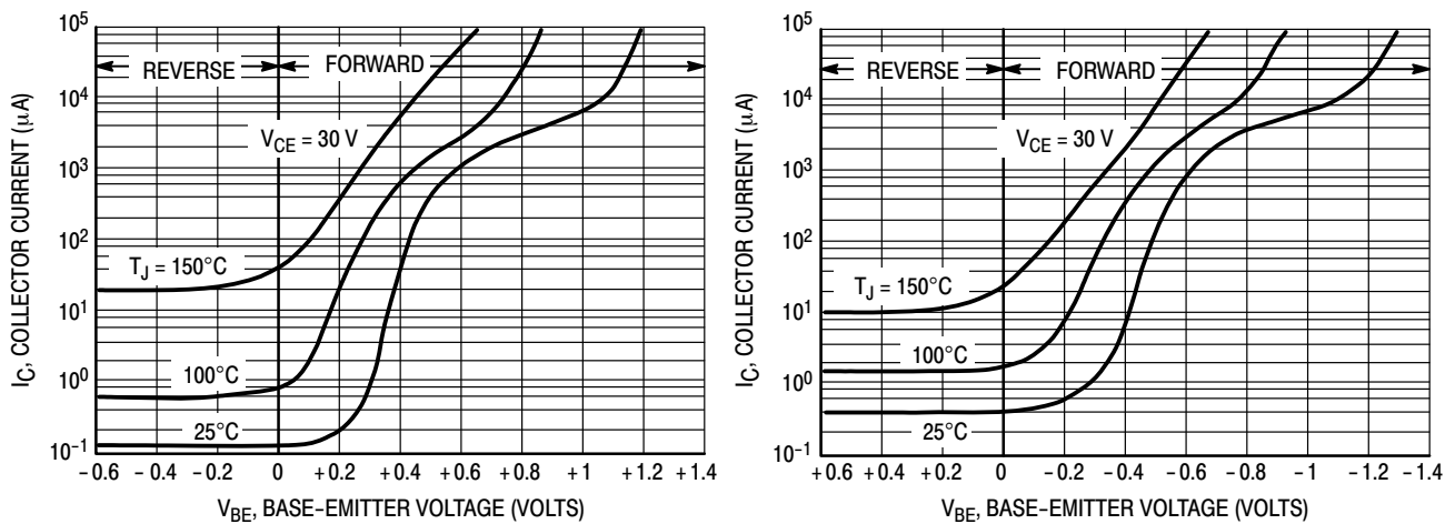
Figure 12. Typical Collector Cut-Off Region
