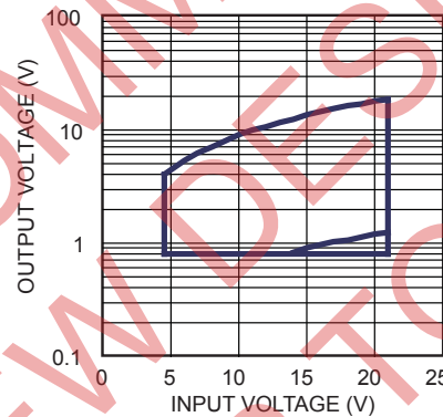
Operating Range
